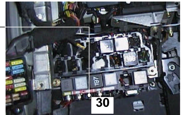
BLK CONNECTOR (98' model) BLU CONNECTOR (from Feb. 99', without comfort close function) (WIRE END)
